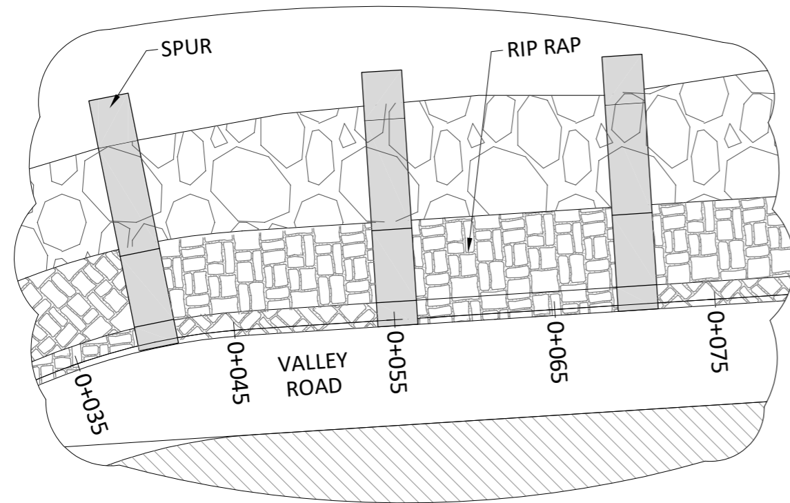
DETAIL A - EMBANKMENT ENLARGED PLAN
