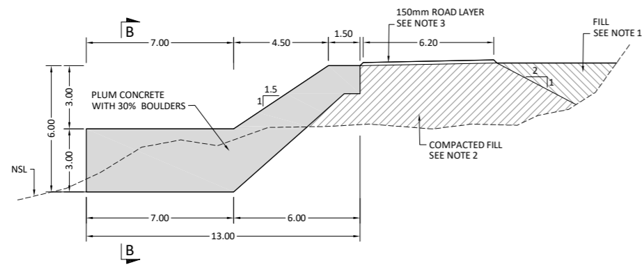
SPUR TYPICAL SECTION CASE - 1
