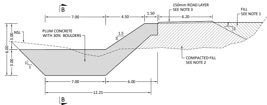
SPUR TYPICAL SECTION CASE - 2
