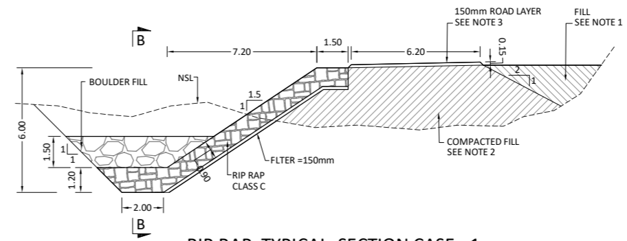
RIP RAP TYPICAL SECTION CASE - 1
