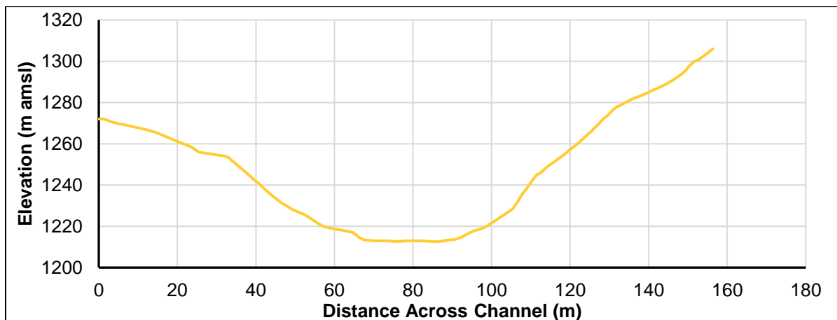
Cross Section 2-2
