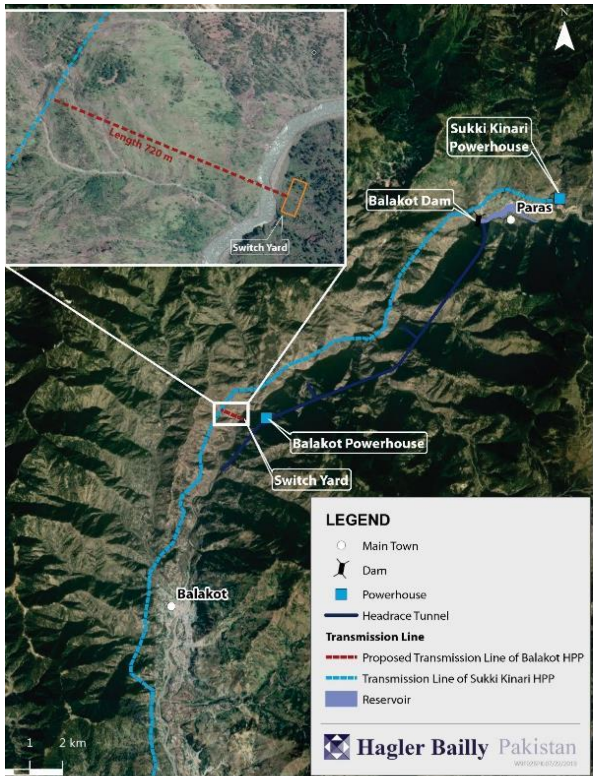
Exhibit 3-24: Schematic of Transmission Line
