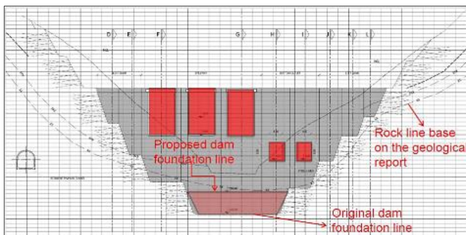
Original Scheme of Spillway and Bottom Outlet
