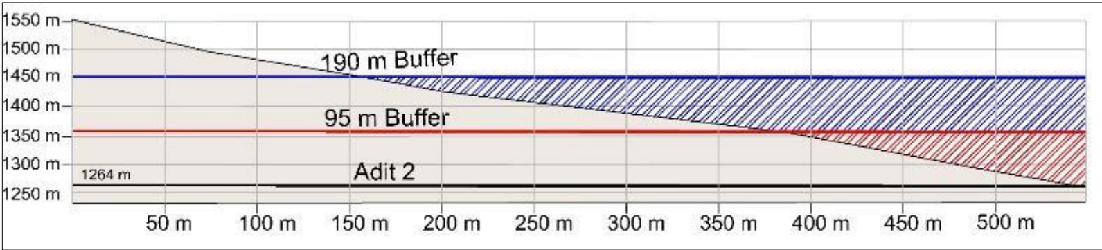
Exhibit 7-18: Depth Profile of Construction Adit 2
