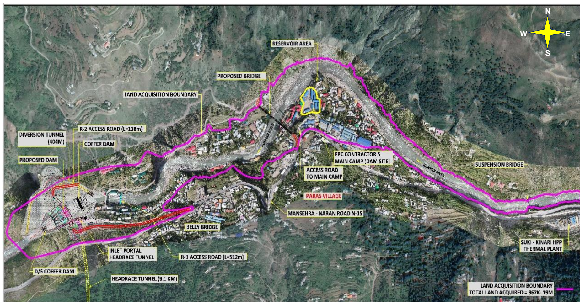
Exhibit 2.5: Project Setting-Dam site
