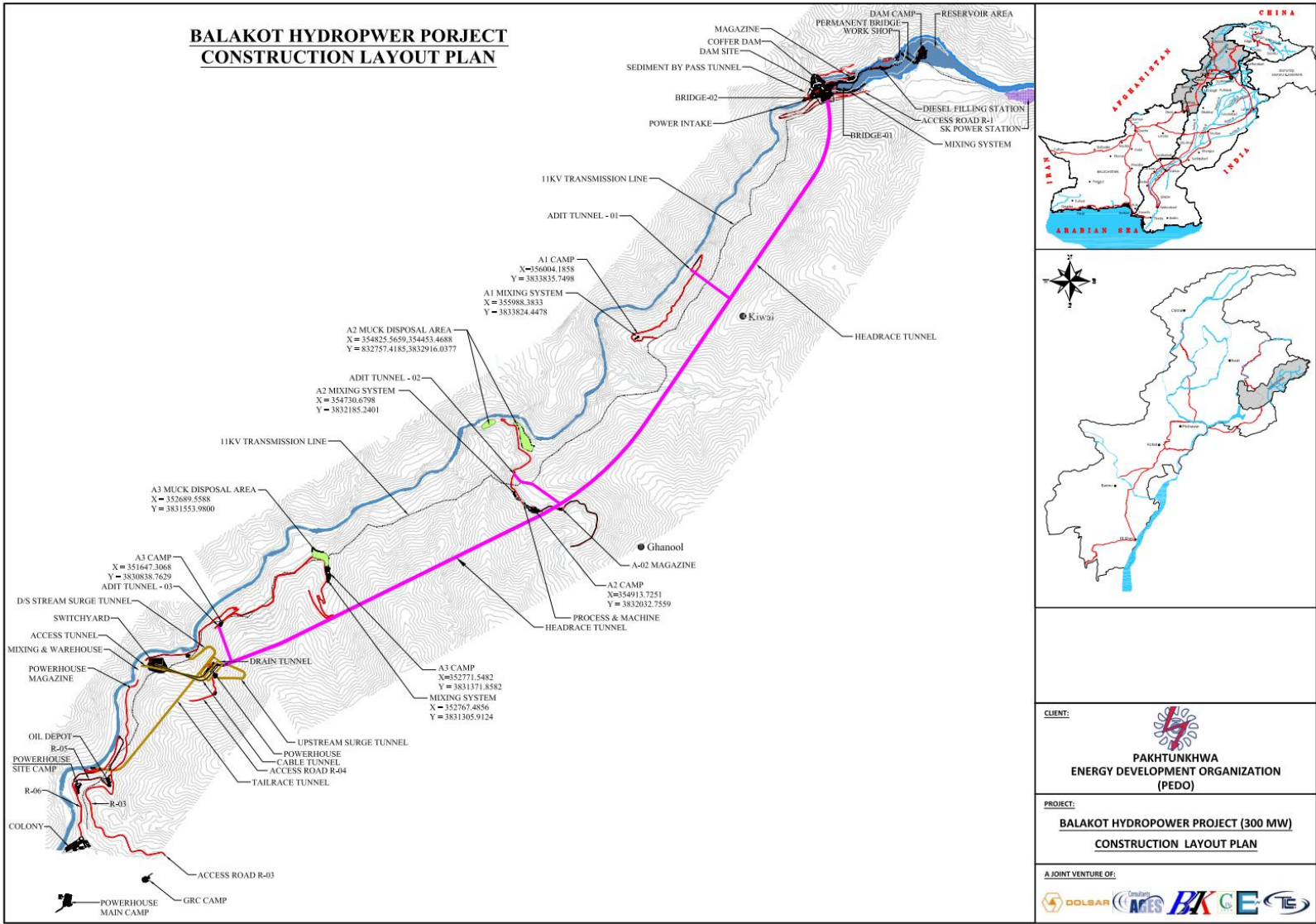
Exhibit 1.3: Project Layout
