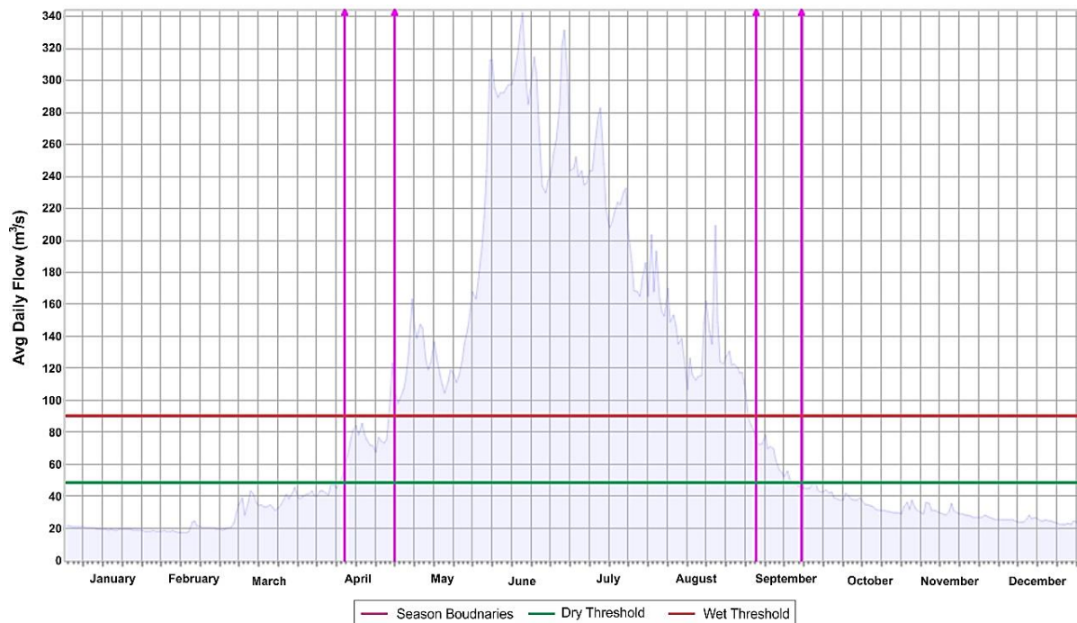
Exhibit 18.15: Hydrograph with Season Delineation at E-Flow Site 2 for Year 1963
