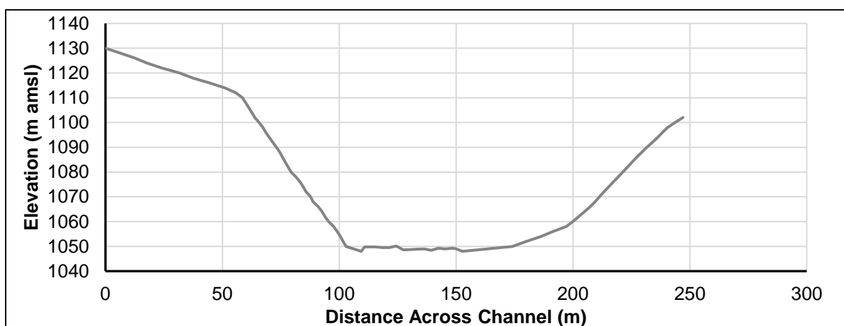
Cross Section 3-1
