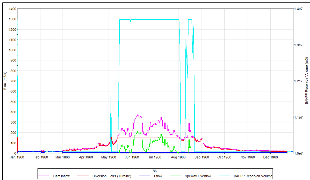
Exhibit 18.28: Dam Volume, Inflows and Outflows Using 10-Day, 90% Dependable Flows –B6 Scenario
