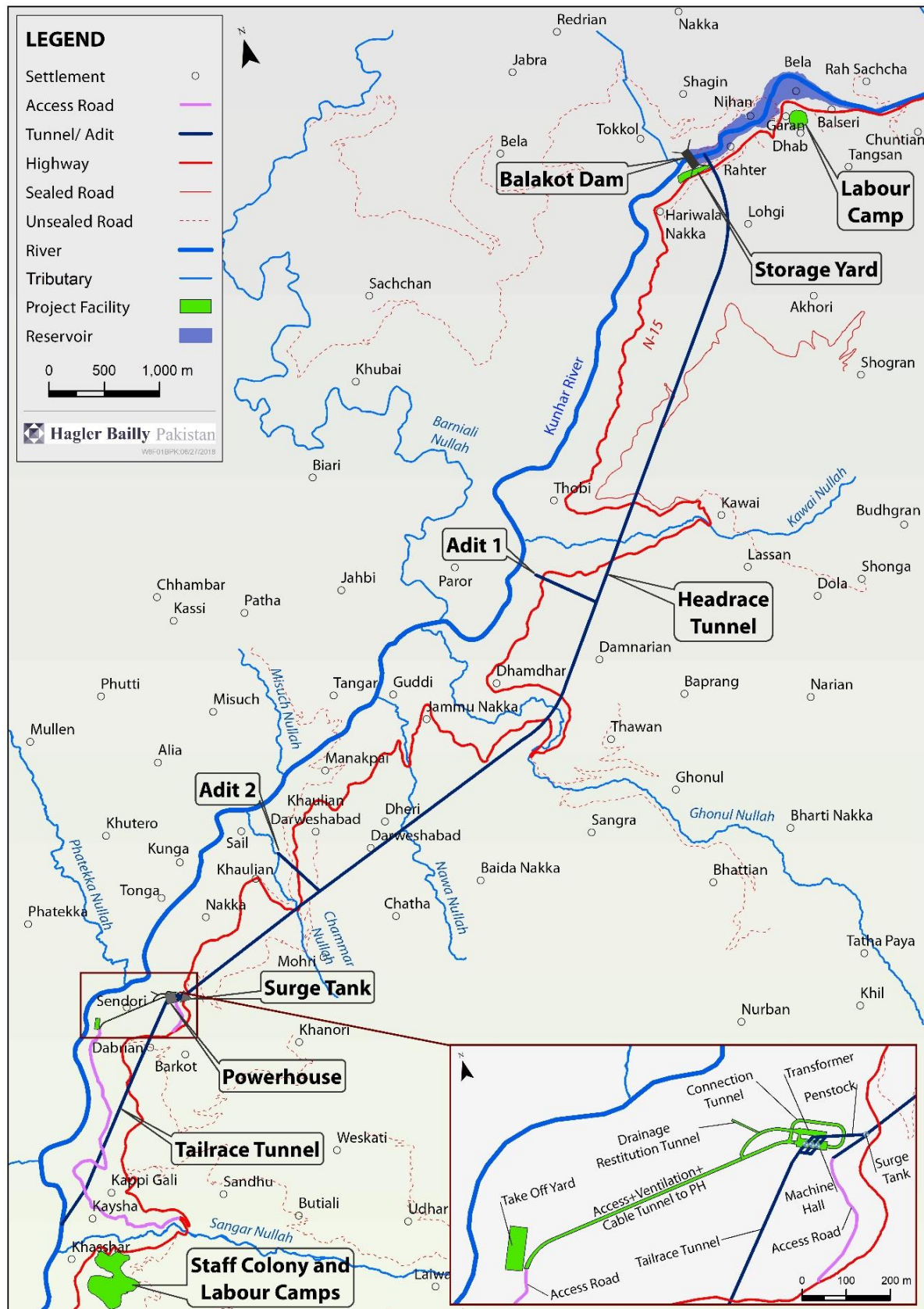
Exhibit 18.69: Project Layout
