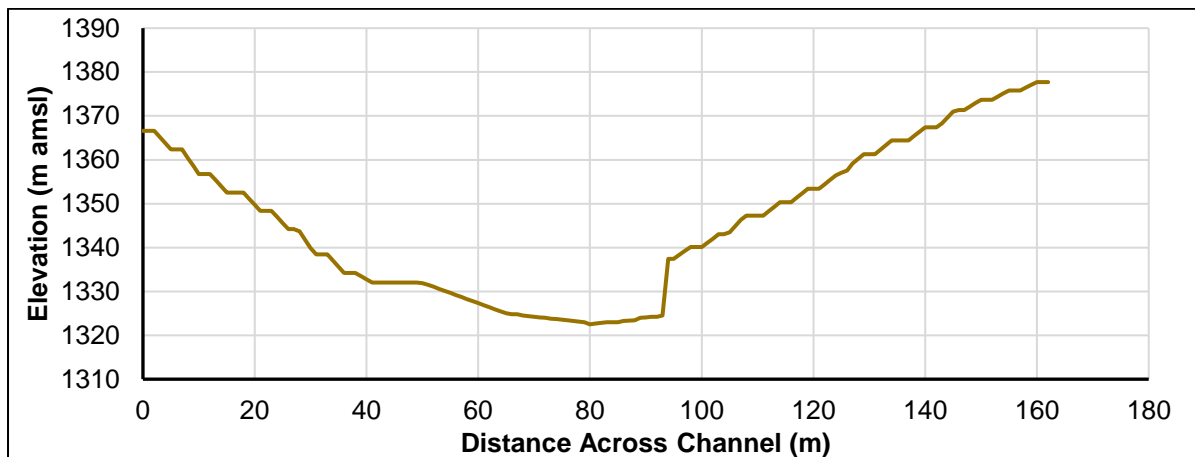
Cross Section 1-1
