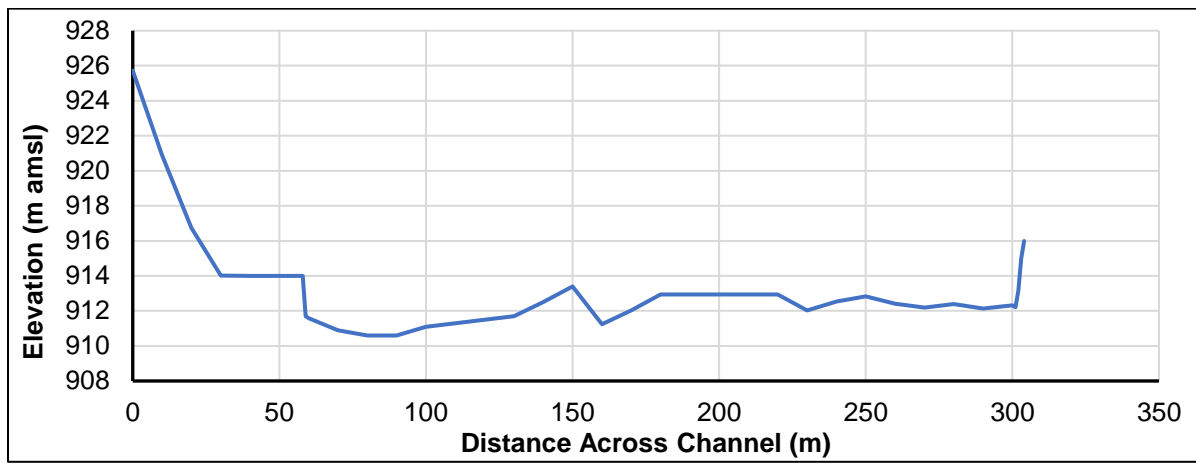
Cross Section 4-2
