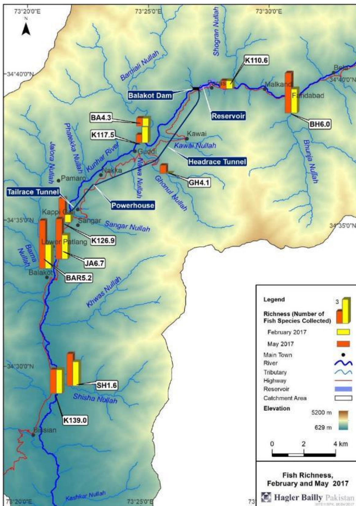
Exhibit 4-96: Comparison of Fish Species Richness, February and May 2017 Survey
