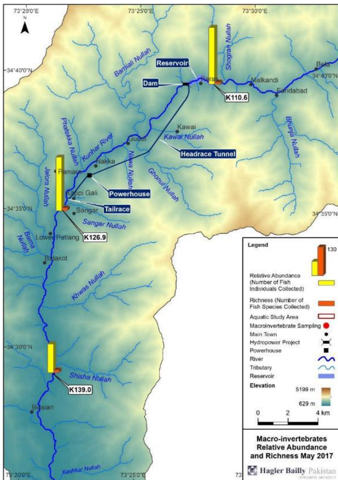
Exhibit 4-109: Distribution of Macro-invertebrate Abundance and Richness, May 2017 Survey
