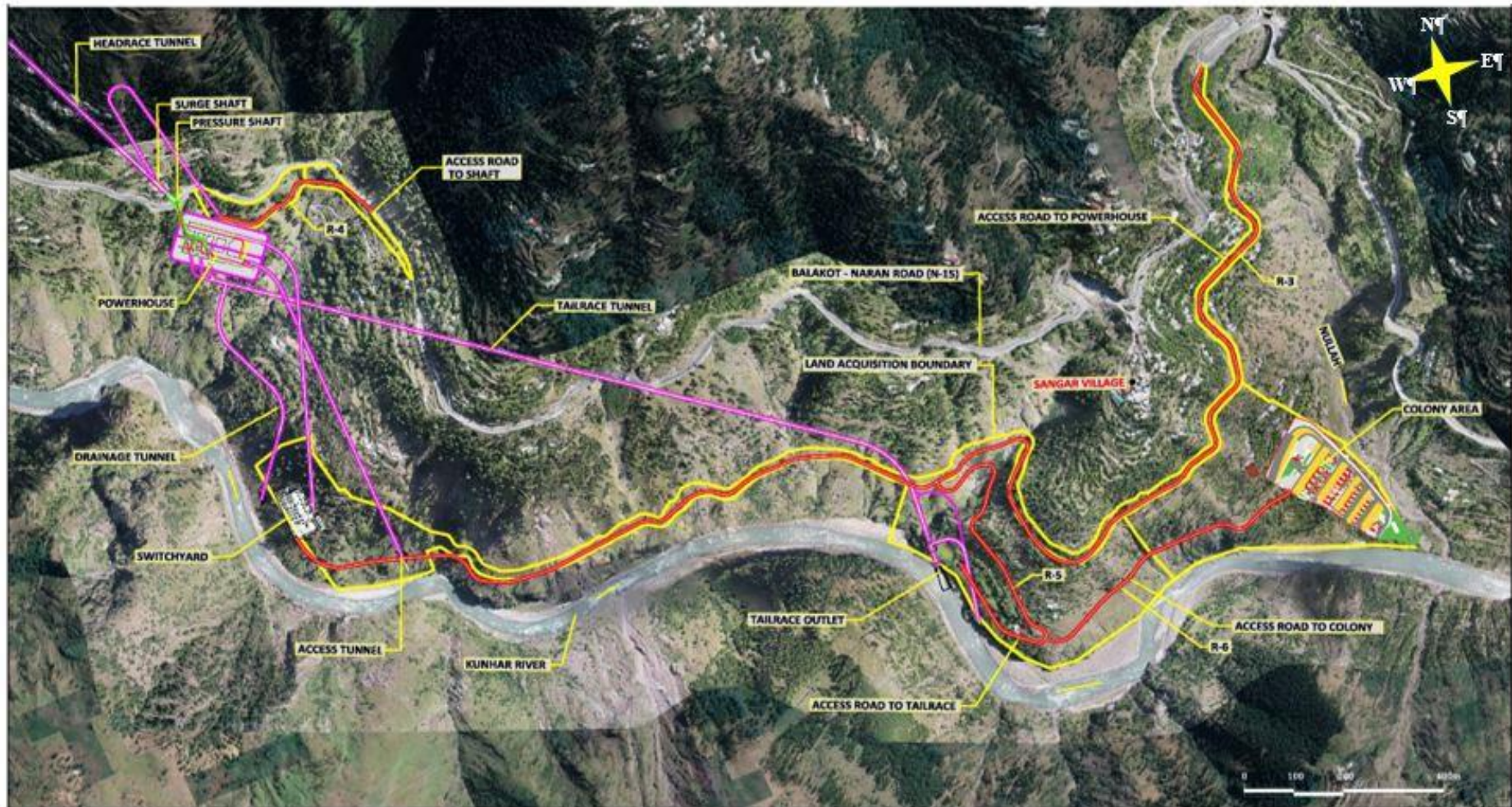
Exhibit 3-6: Project Setting- Powerhouse and Colony Sites
