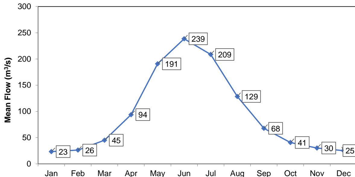
Exhibit 18.8: Mean Monthly Flow at Talhata (1995-2010)
