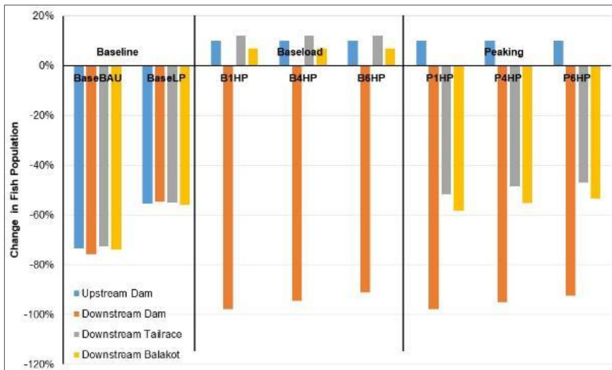
Exhibit 5-9: Kashmir Hillstream Loach Predicted Change in Population
