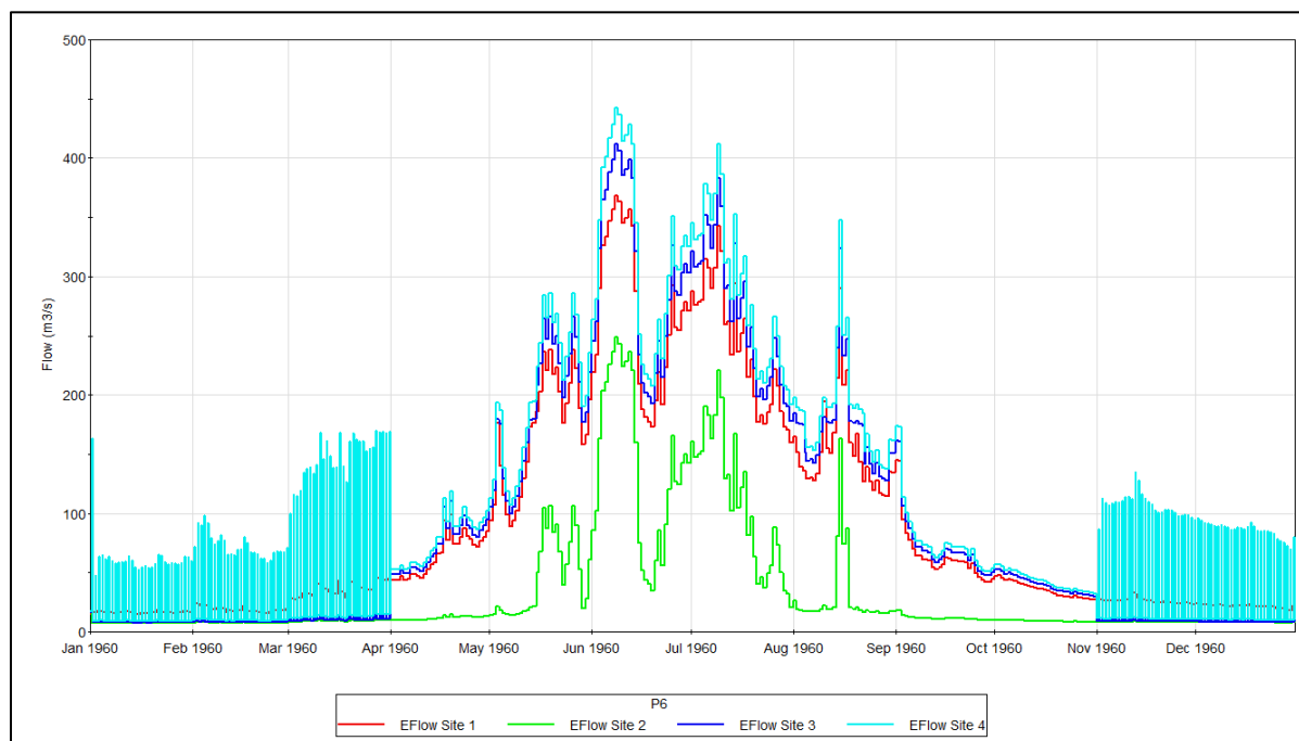
Exhibit 18.24: Flow at EF Sites with Dam Operation – P6 Scenario
