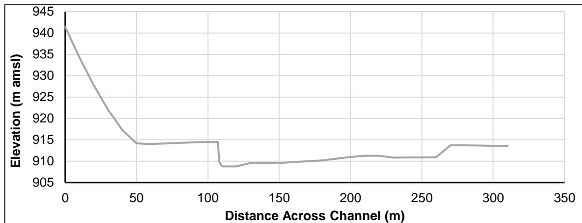
Cross Section 4-1
