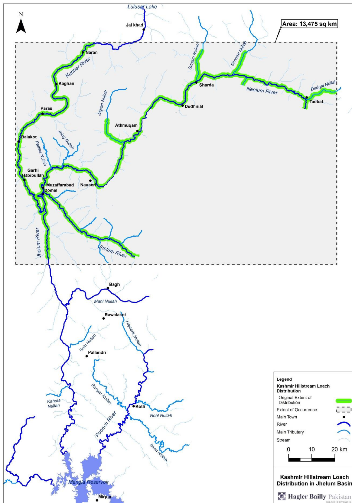
Exhibit 11.5: Distribution of the Kashmir Hillstream Loach
