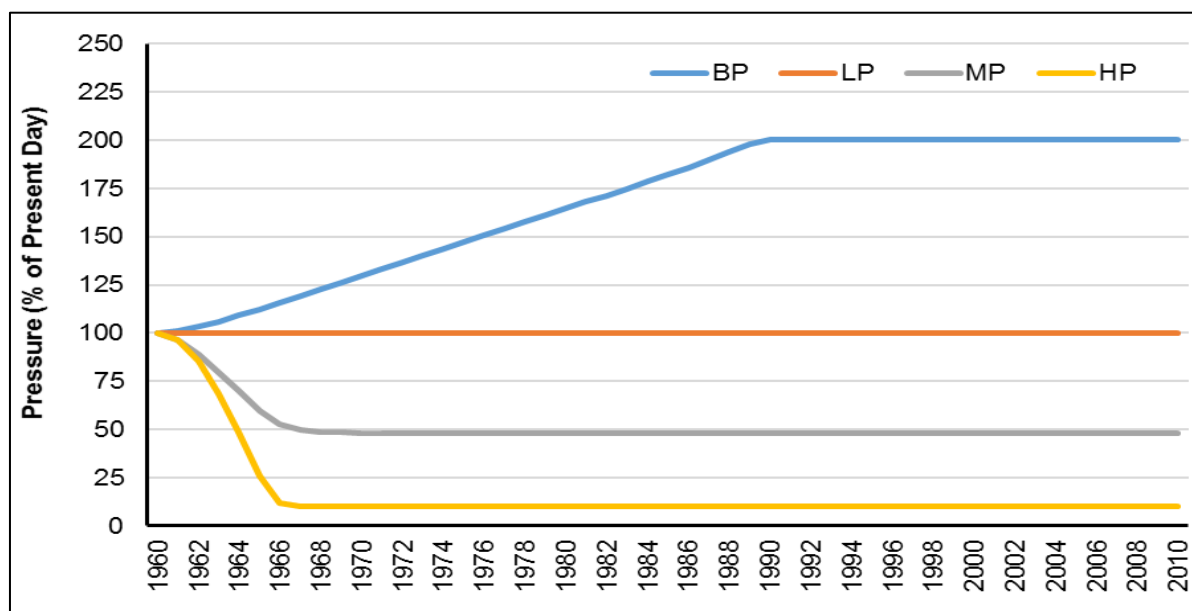
Exhibit 3.2: Pressure Levels over Time as Incorporated into DRIFT
