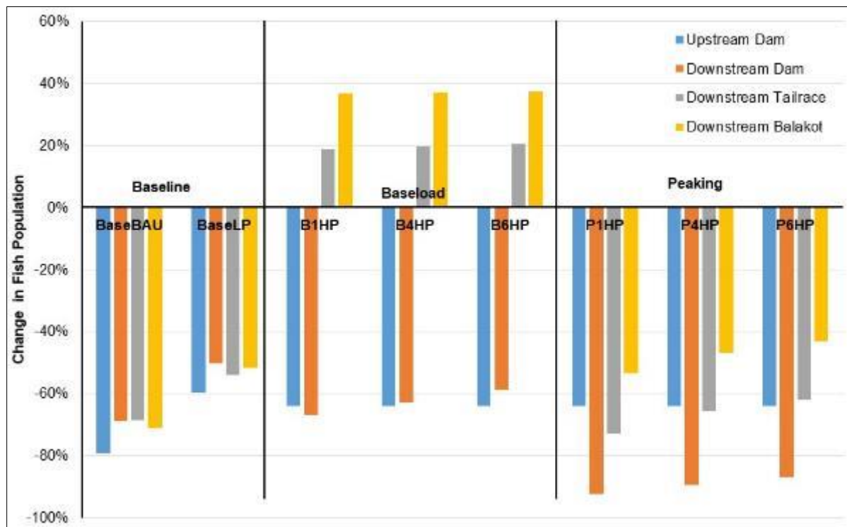
Exhibit 5-5: Alwan Snow Trout Predicted Change in Population
