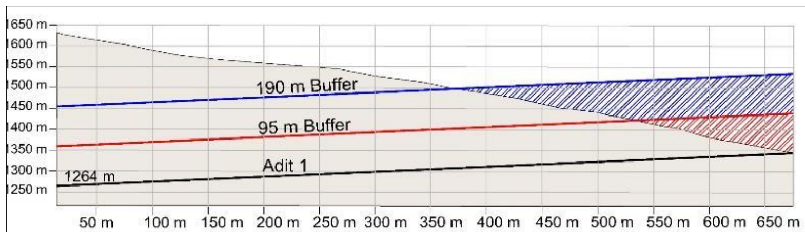
Exhibit 7-17: Depth Profile of Construction Adit 1
