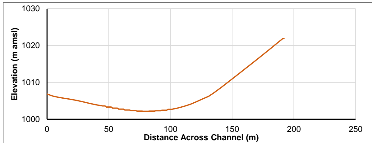
Cross Section 3-5
