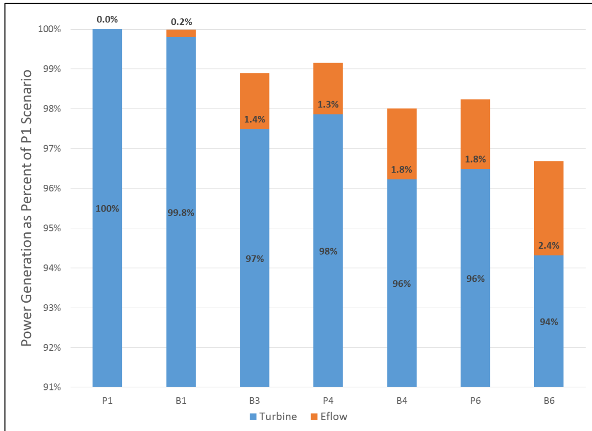
Exhibit 18.32: Power Generation
