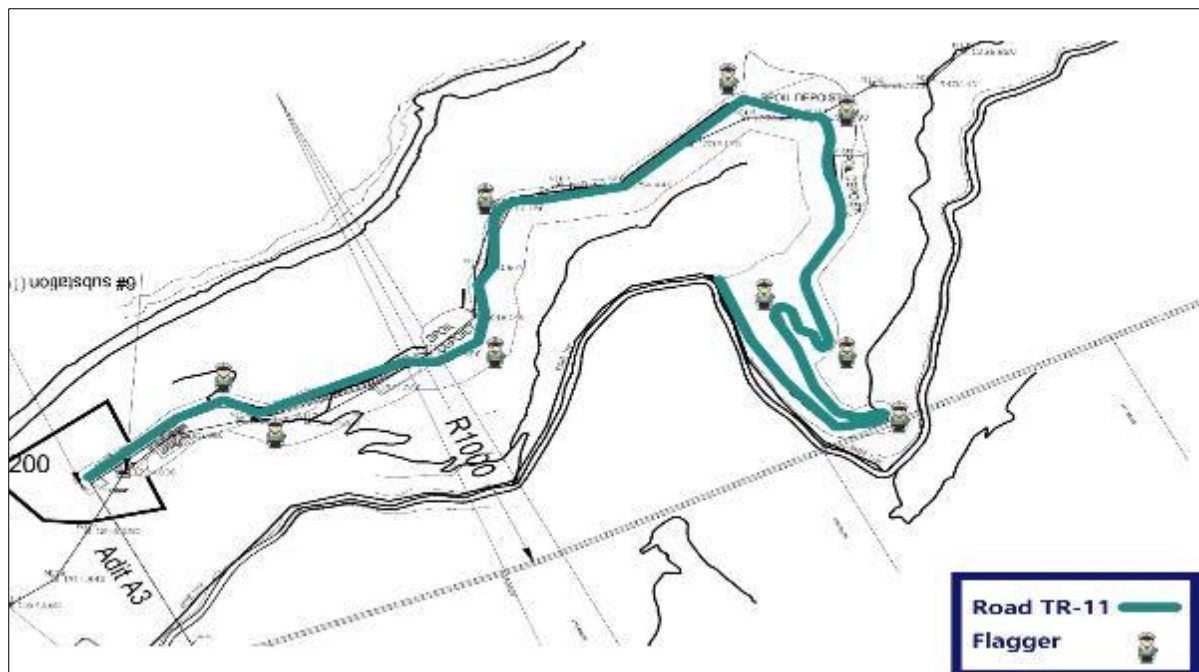
Exhibit 3-14: Access Road Layout at Adit-3
