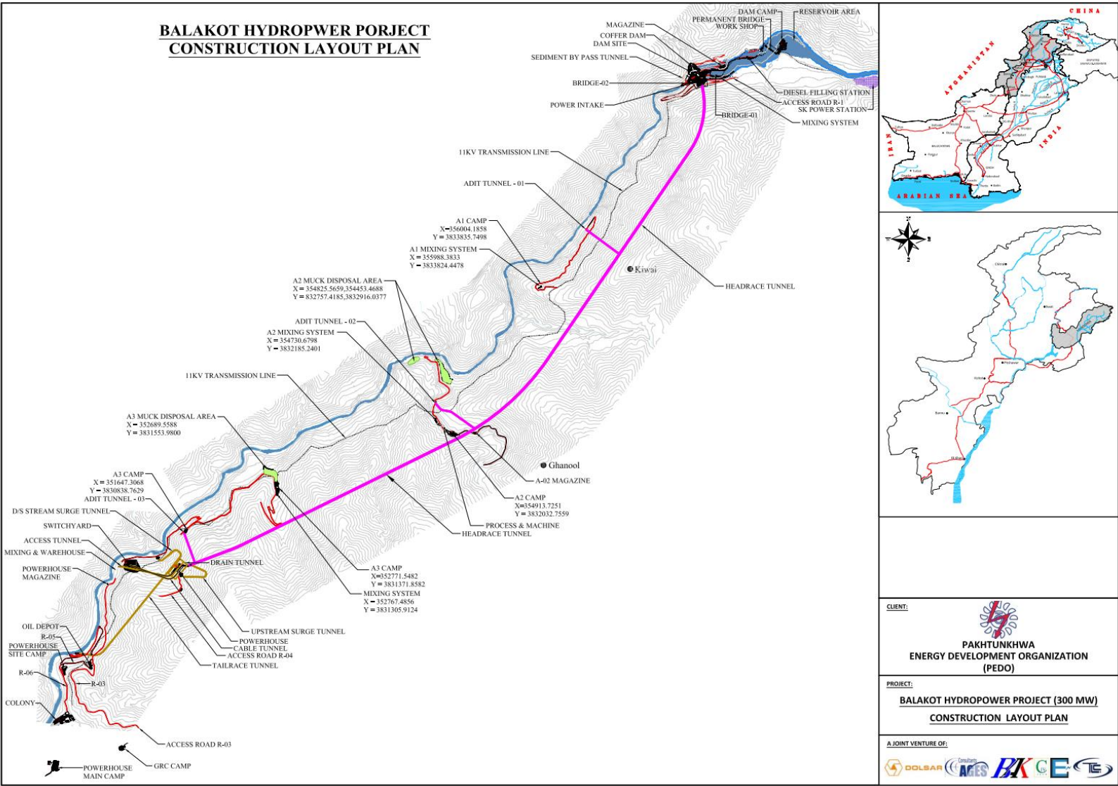
Exhibit 1-5: Project Layout
