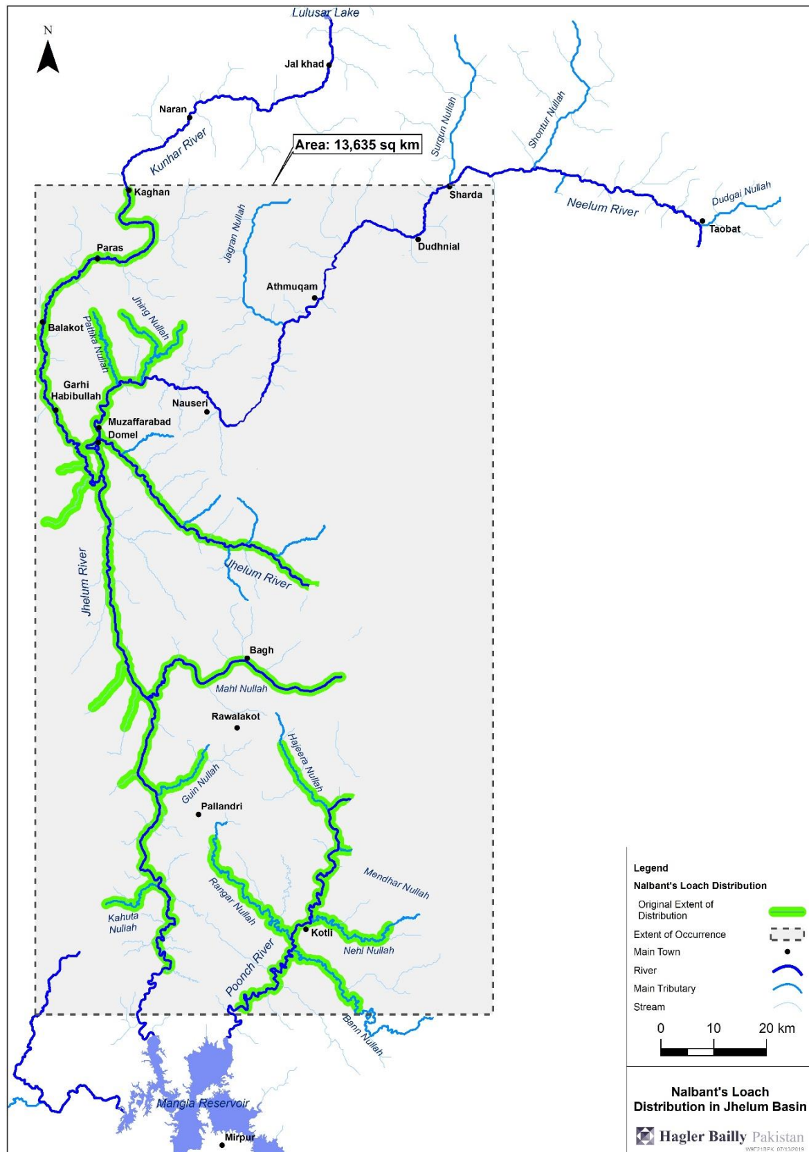
Exhibit 11.4: Distribution of the Nalbant's Loach
