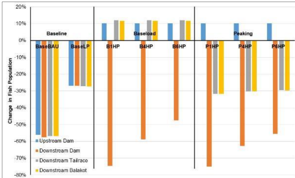
Exhibit 5-7: Nalbant's Loach Predicted Change in Population
