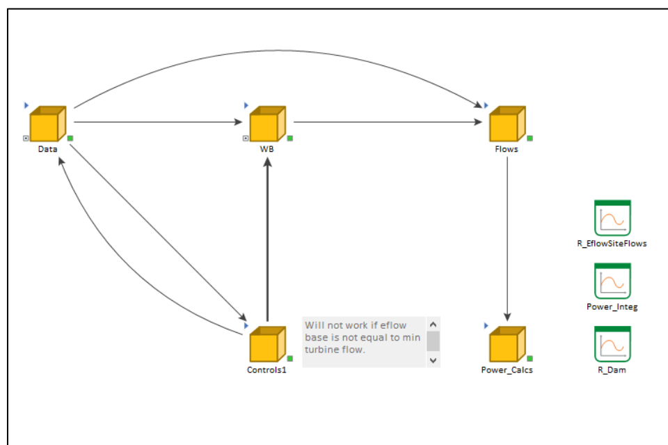
Exhibit 18.16: Screenshots Parts of GoldSim® Model
