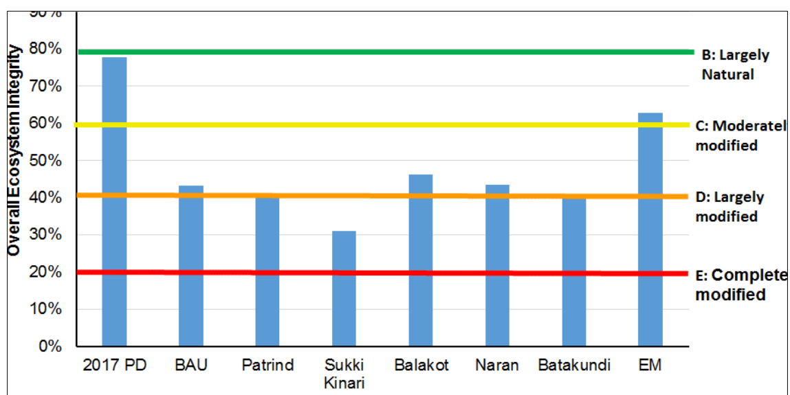
Exhibit 7-45: Predicted Ecosystem Integrity in the CIA Study Area with Sequential Implementation of Hydropower Projects
