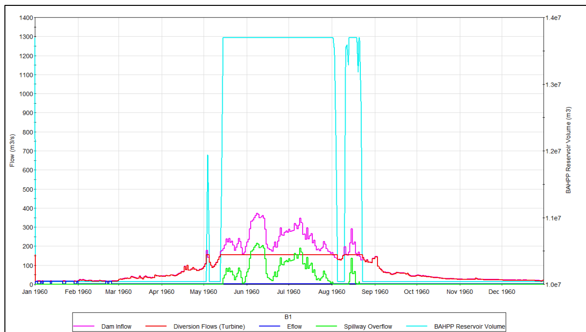
Exhibit 18.25: Dam Volume, Inflows and Outflows using 10-Day, 90% Dependable Flows –B1 Scenario
