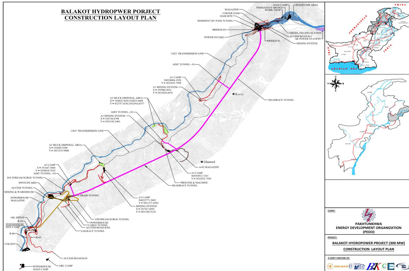
Exhibit 2.4: Project Layout Map
