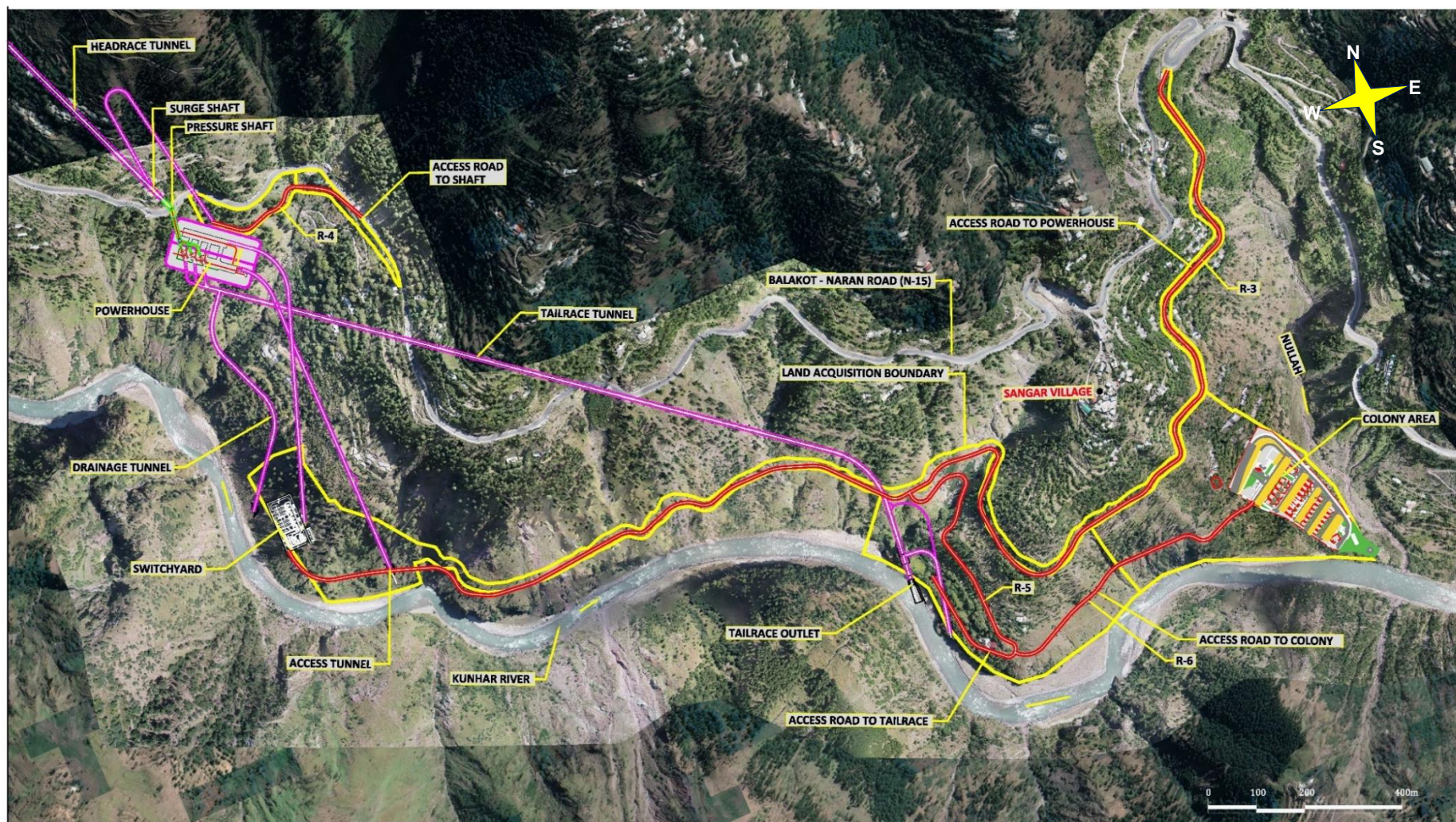
Exhibit 2.6: Project Setting-Powerhouse and Colony sites
