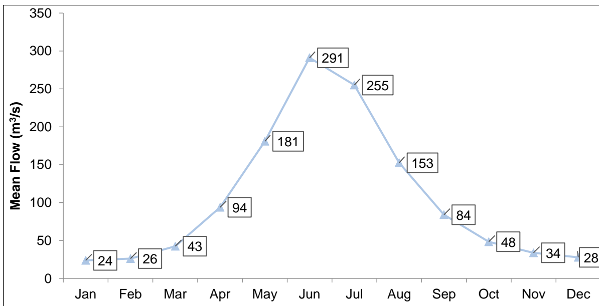
Exhibit 18.7: Mean Monthly Flow at Gari Habibullah (1960-1994)
