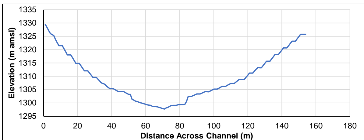
Cross Section 1-2
