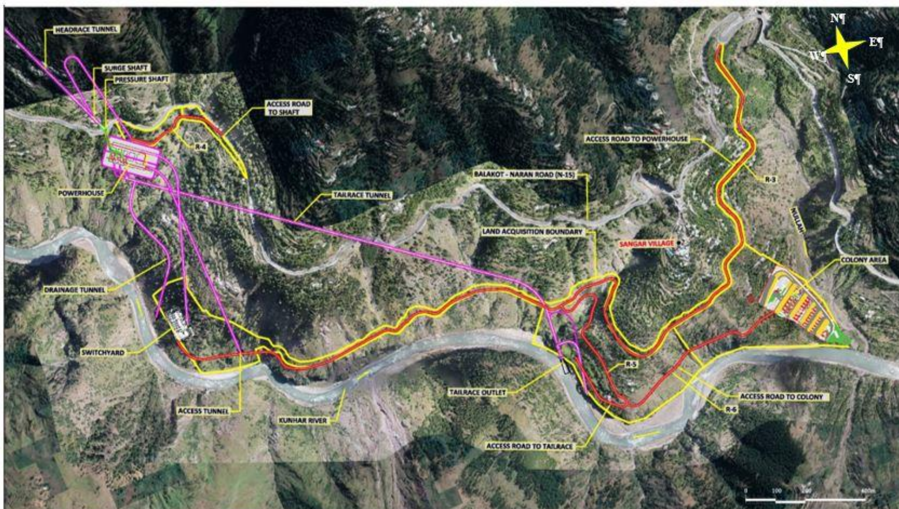
Exhibit 1-7: Project Setting- Powerhouse and Colony Sites
