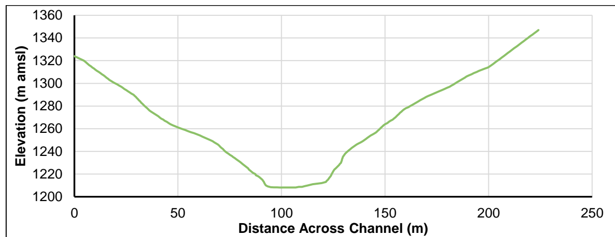
Cross Section 2-4
