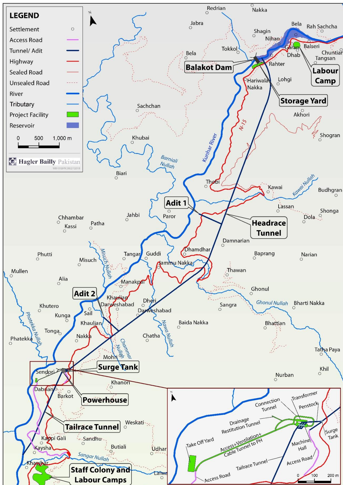
Exhibit 3: Project Layout
