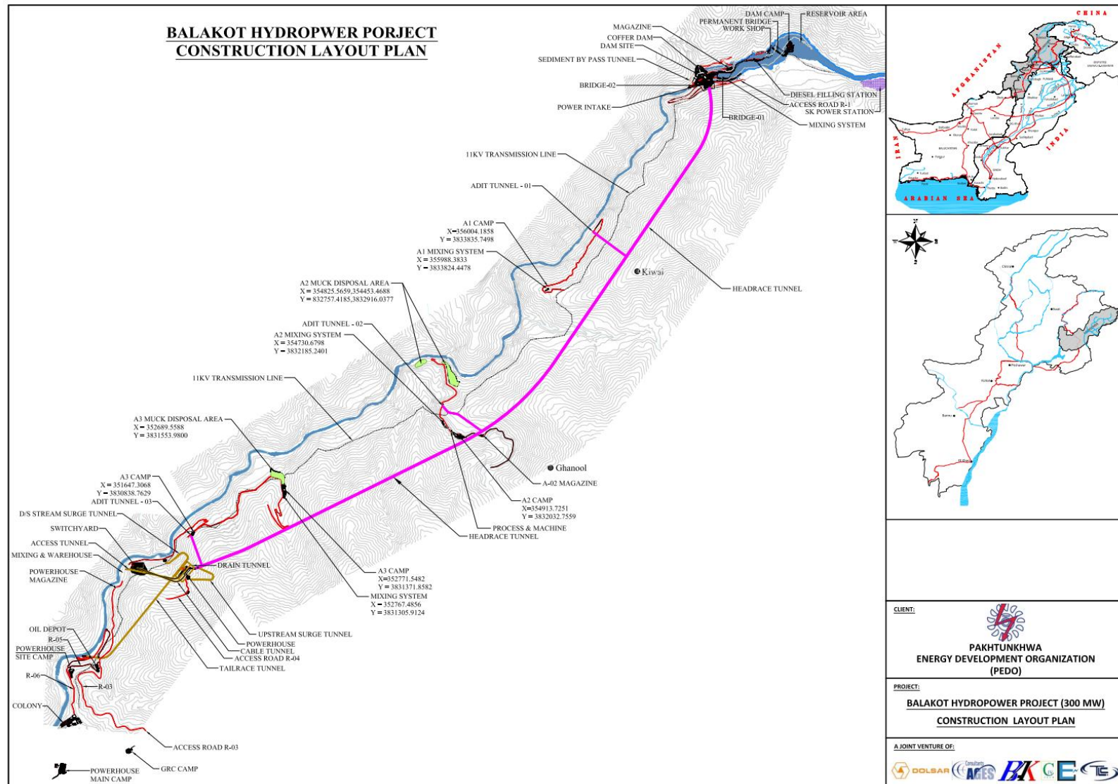
Exhibit 3-4: Project Layout
