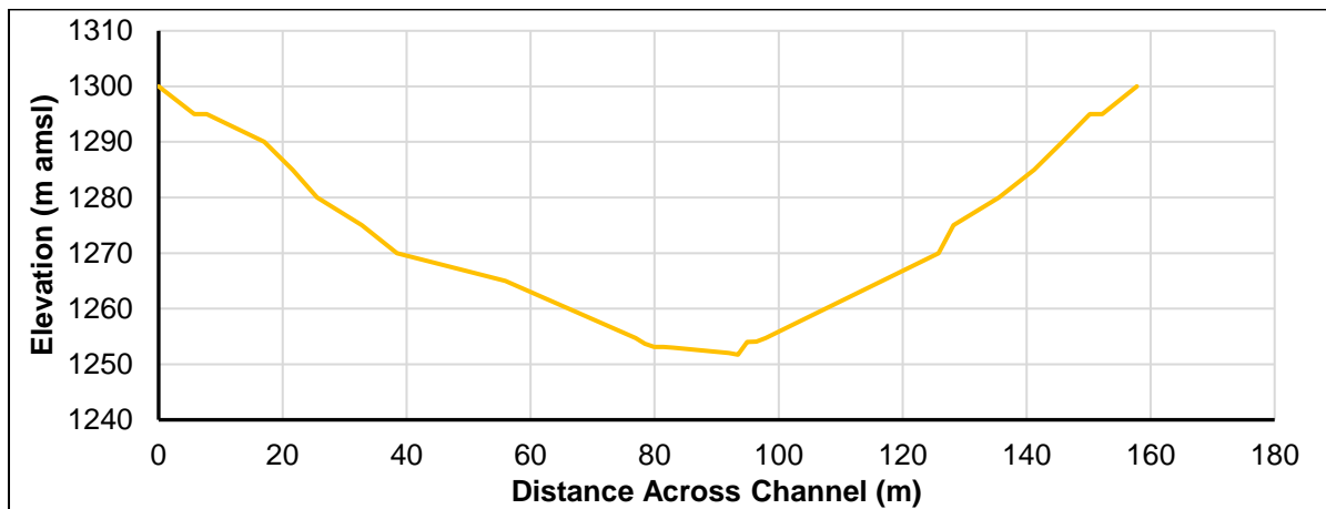
Cross Section 1-5
