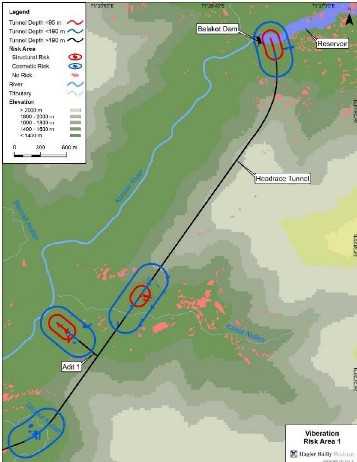
Exhibit 7-19: Vibration Risk Area 1
