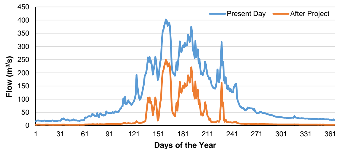
Exhibit 7-28: Comparison of Baseline and Post Project Hydrograph in the Low Flow Section, 1960
